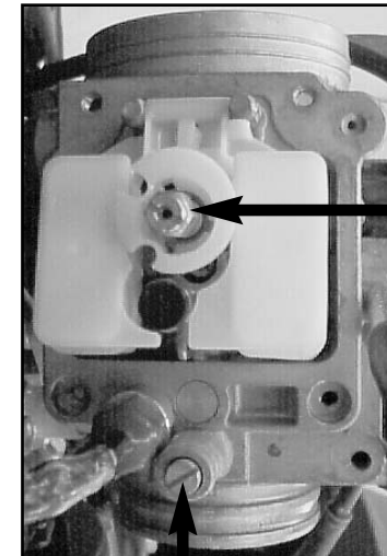
Fuel Mixture Screw
